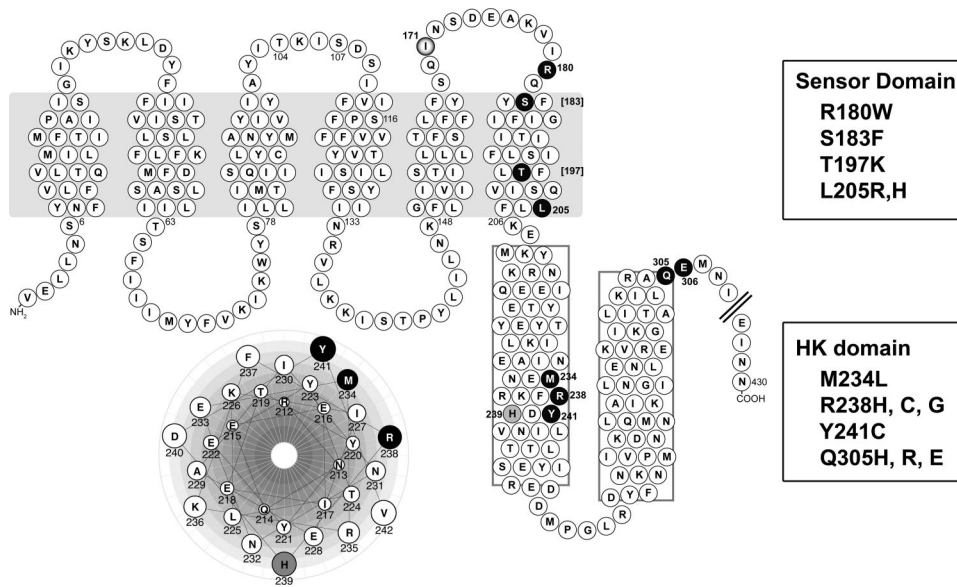
Fig. 1. AgrC-I topology, domain prediction, and mutagenized residues. AgrC-I is a 430-aa protein with a polytopic TM sensor domain (7, 28) and a cytoplasmic HK domain, which is further divided into the DHP and CA subdomains. Two cytoplasmic regions with high \alpha -helical propensity predicted to form the DHP domain are boxed. The active site histidine (H239) is shown in gray. Residues analyzed in this study in which mutation (listed at right) resulted in constitutive activity are shown in black. Residue I171, in which mutation resulted in broadened specificity, is shown in spherical relief. ( Inset ) Helical wheel analysis of a region within the first predicted DHP \alpha -helix.
